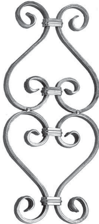
Art. I300/4 Ø 12 x 6 mm H 380 mm L 175 mm
